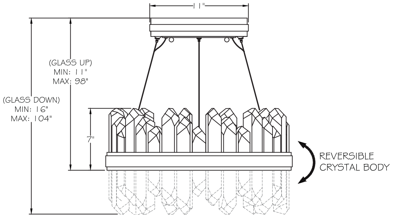
FRONT VIEW
